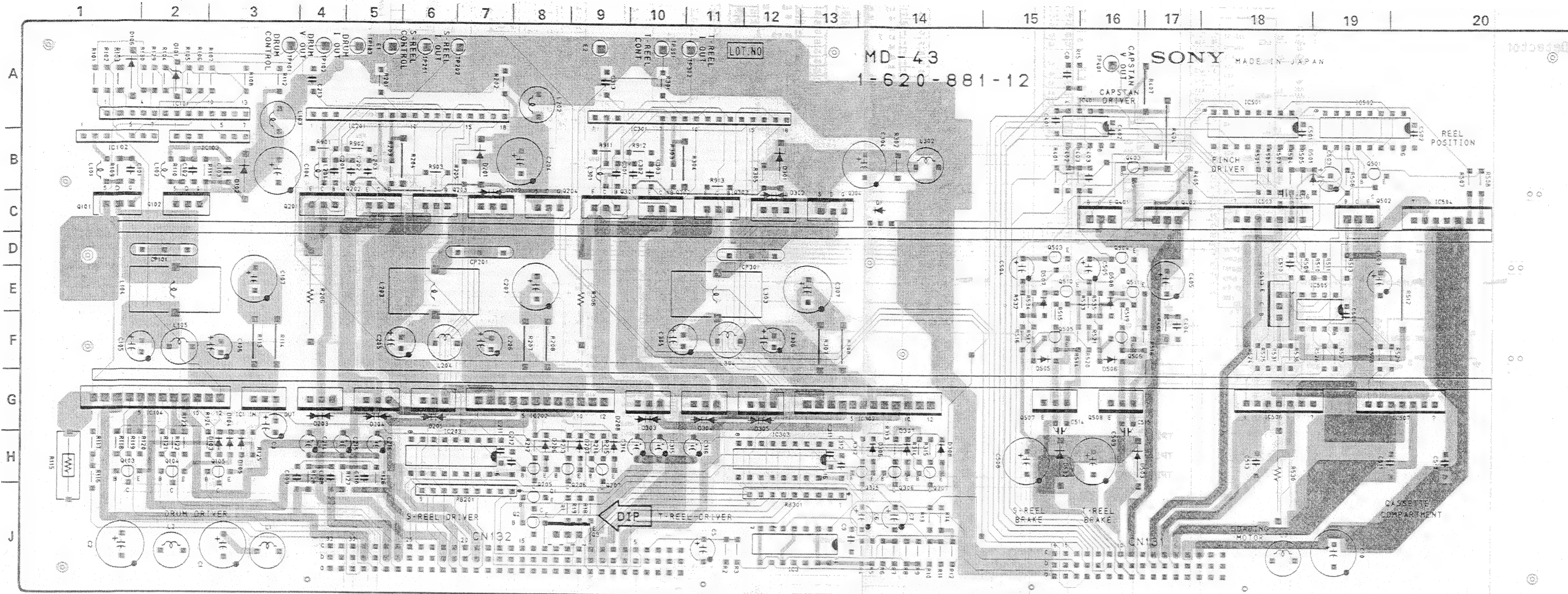
1-620-881-12 COMPONENT SIDE
